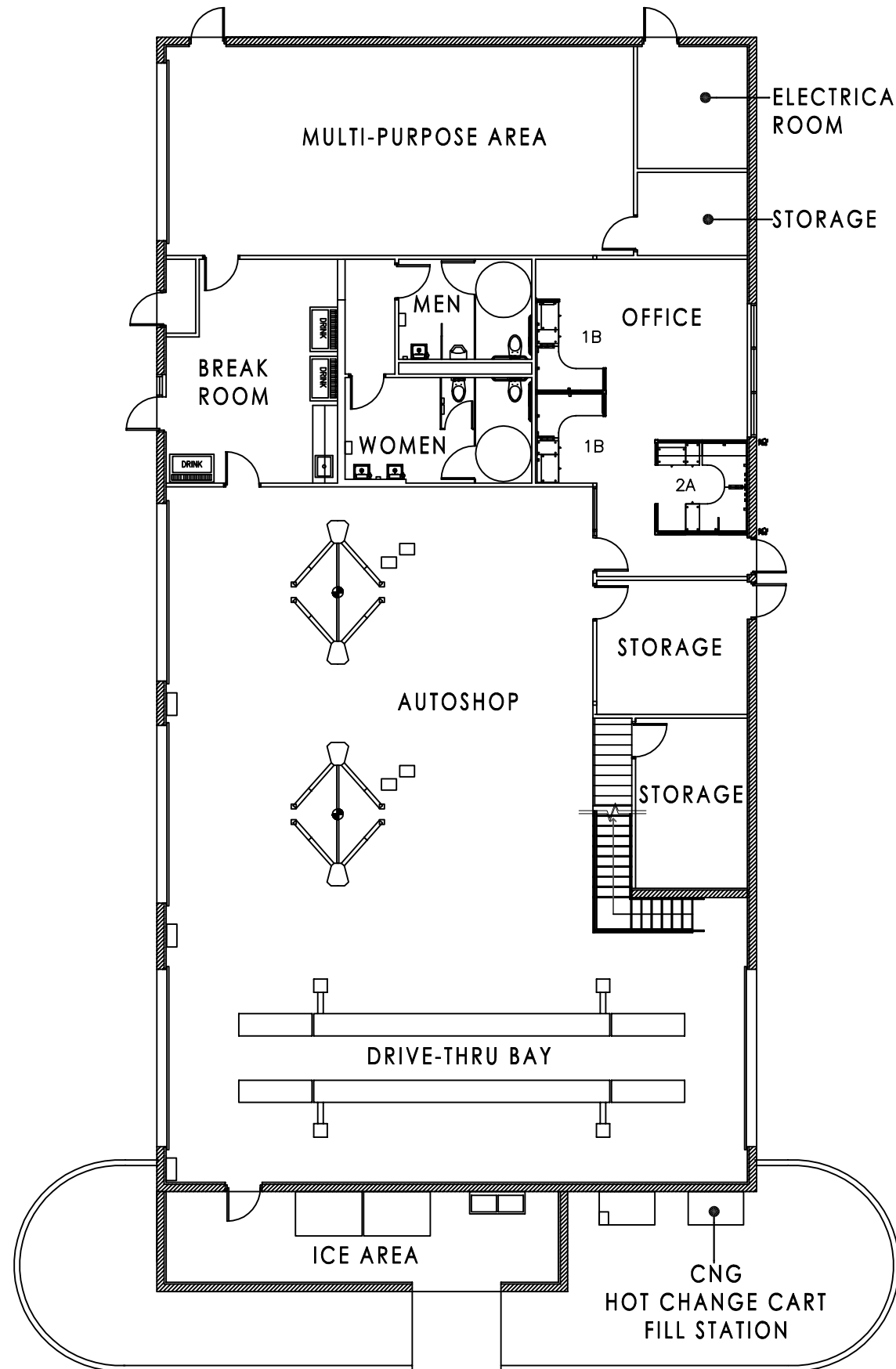
AUTOSHOP FIRST FLOOR PLAN
