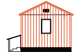
RIGHT ELEVATION – TYPE B
