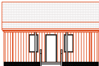
FRONT ELEVATION – TYPE C
