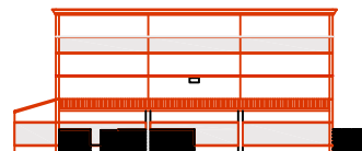
SOUTH ELEVATION - AUTOSHOP & PRE-FABRICATION SHOP
