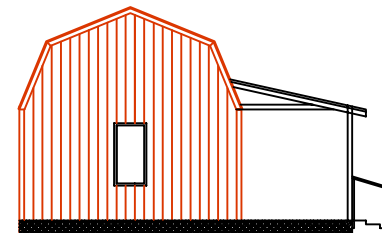
LEFT ELEVATION – TYPE C
