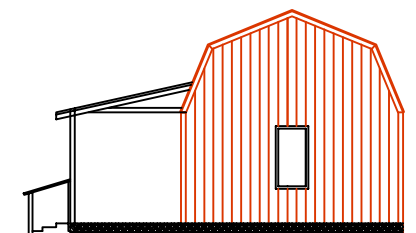
RIGHT ELEVATION – TYPE C
