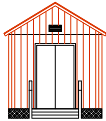
FRONT ELEVATION – TYPE A
